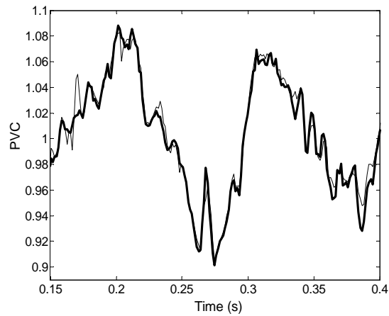
Fig. 5: Fragment of PVC courses. Solid line corresponds to PVC evaluated from single track. Solid thin line corresponds to PVC evaluated from a set of tracks.
