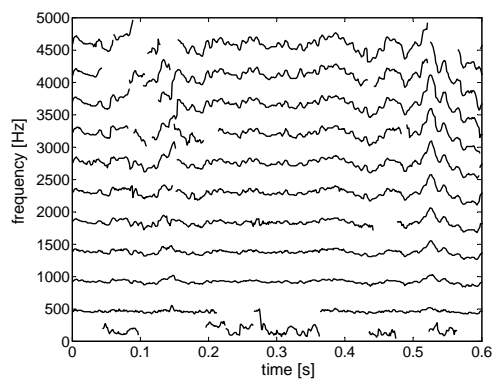
(b) Distorted frequency tracks from a wow-contaminated sound.
