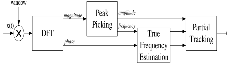
Fig. 3: Block diagram of sinusoidal modeling approach for wow evaluation.
