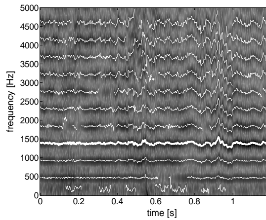
Fig. 4: Tracks evaluated by the algorithm. The track depicted by a bold line is used in further experiments.
